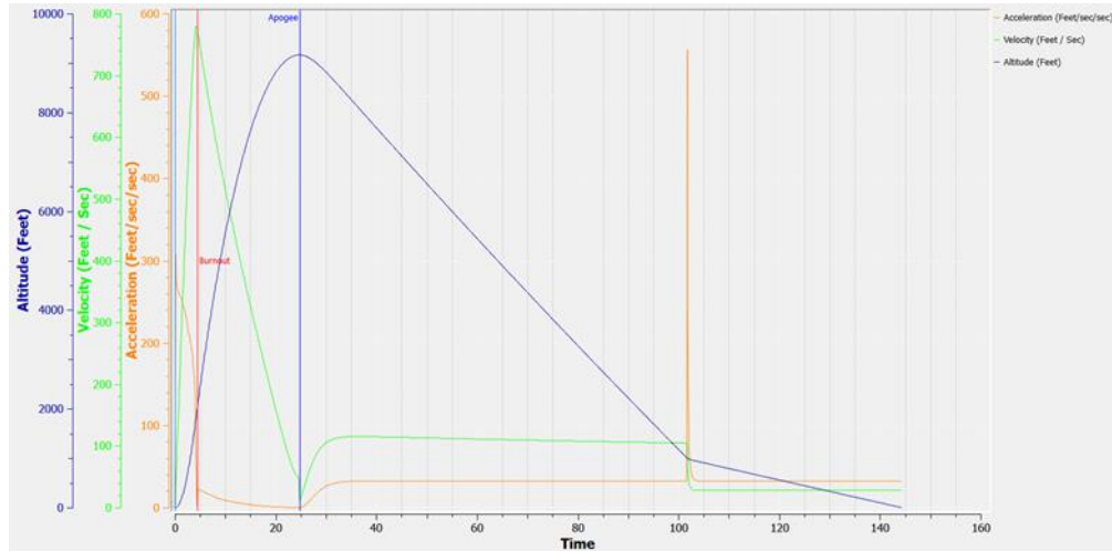
Figure 3 RockSim Flight Trajectory Analysis:
