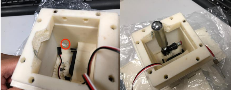
Figure 6: Location of the inflation hole and correct placement of the cannister.
