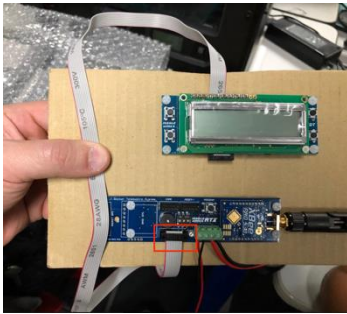
Figure 11: Connection of the LCD screen to the base RT x Module
