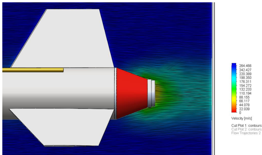
Figure 16: CFD Boattail
