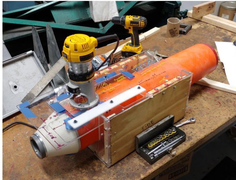
Figure 6: Tube Slotting Jig
