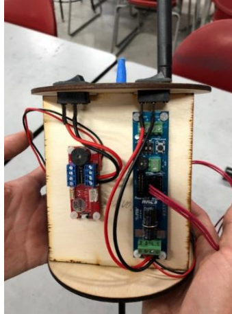
Figure 18: StratoLoggerCF (left) and RRC3 (right) altimeters
