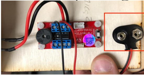
Figure 16: Strato-logger power source connector
