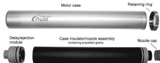
Figure 1. Pro54 Components
