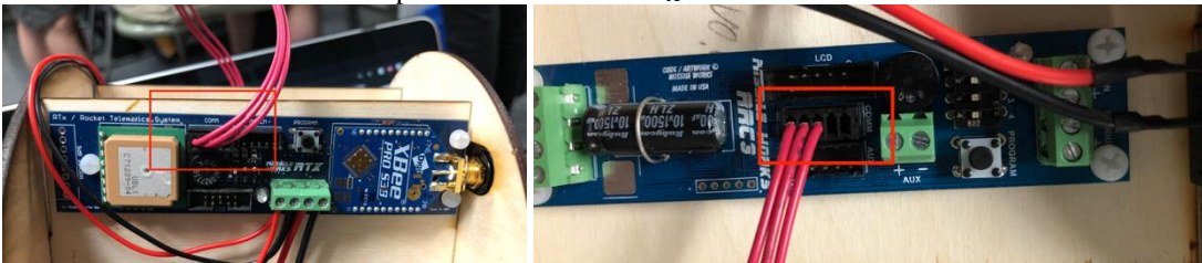
Figure 12: Comm port connection on the Rocket RT x module (left) and the RRC3 Altimeter(right).
