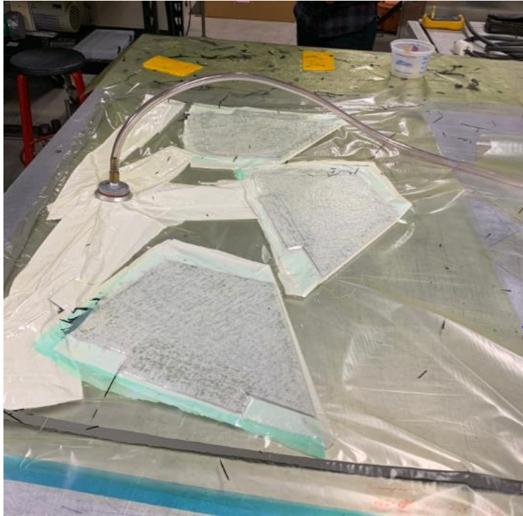
Figure 9: Composite Fin Layup
