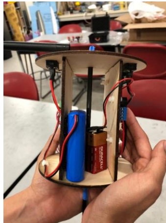
Figure 20: Avionics Bay Battery Compartment
