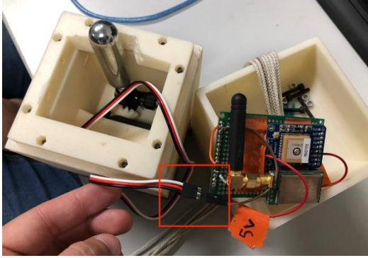
Figure 7: Connection of 5V and Ground wires to the servo motor.
