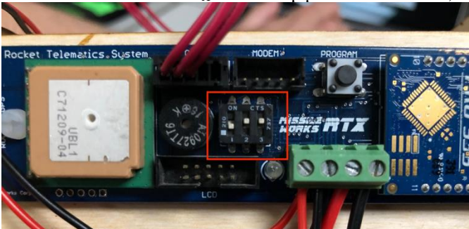
Figure 13: Dip switch settings set to OFF, ON, ON for the Base RT x module
