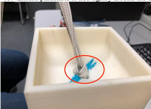
Figure 10: Preferred fastening of parachute to payload.
