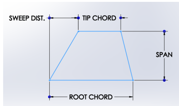
Figure 7: Fin Dimensions Diagram
