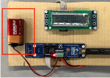
Figure 15: Connection of the 9V power source to the Base RTx Module.
