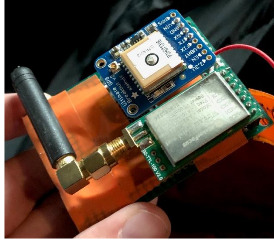
Figure 25: GPS module (upper left) and LoRa radio transmitter (lower right)
