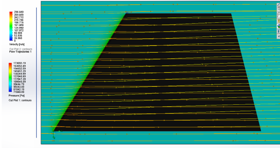
Figure 11: CFD Fin Side View
