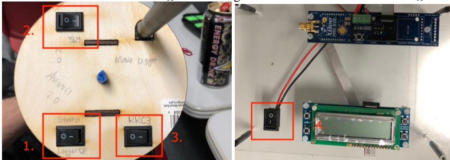
Figure 17: Order of switches for powering up the avionics system.
