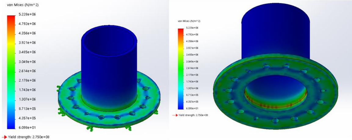
Figure 15: Top and Bottom View Thrust Plate Stress Analysis
