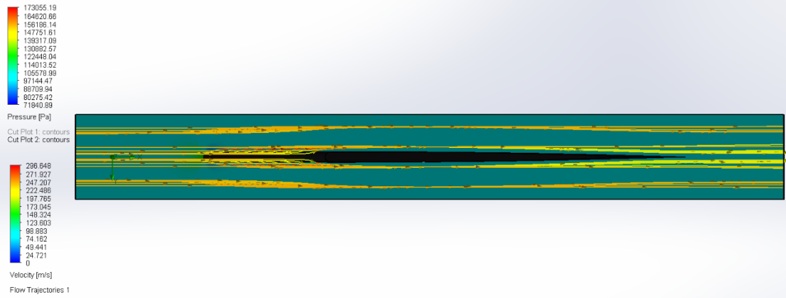
Figure 12: CFD Fin Top View
